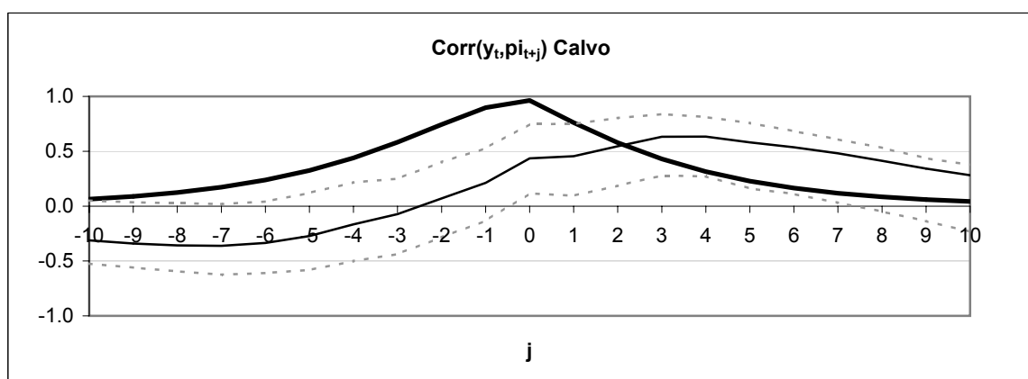
Figure 6: Dynamic Cross-Correlations
