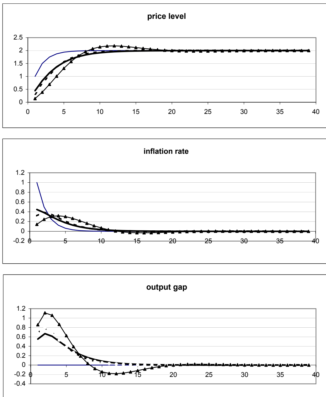
Figure 1: Impulse Responses - Theoretical Model
