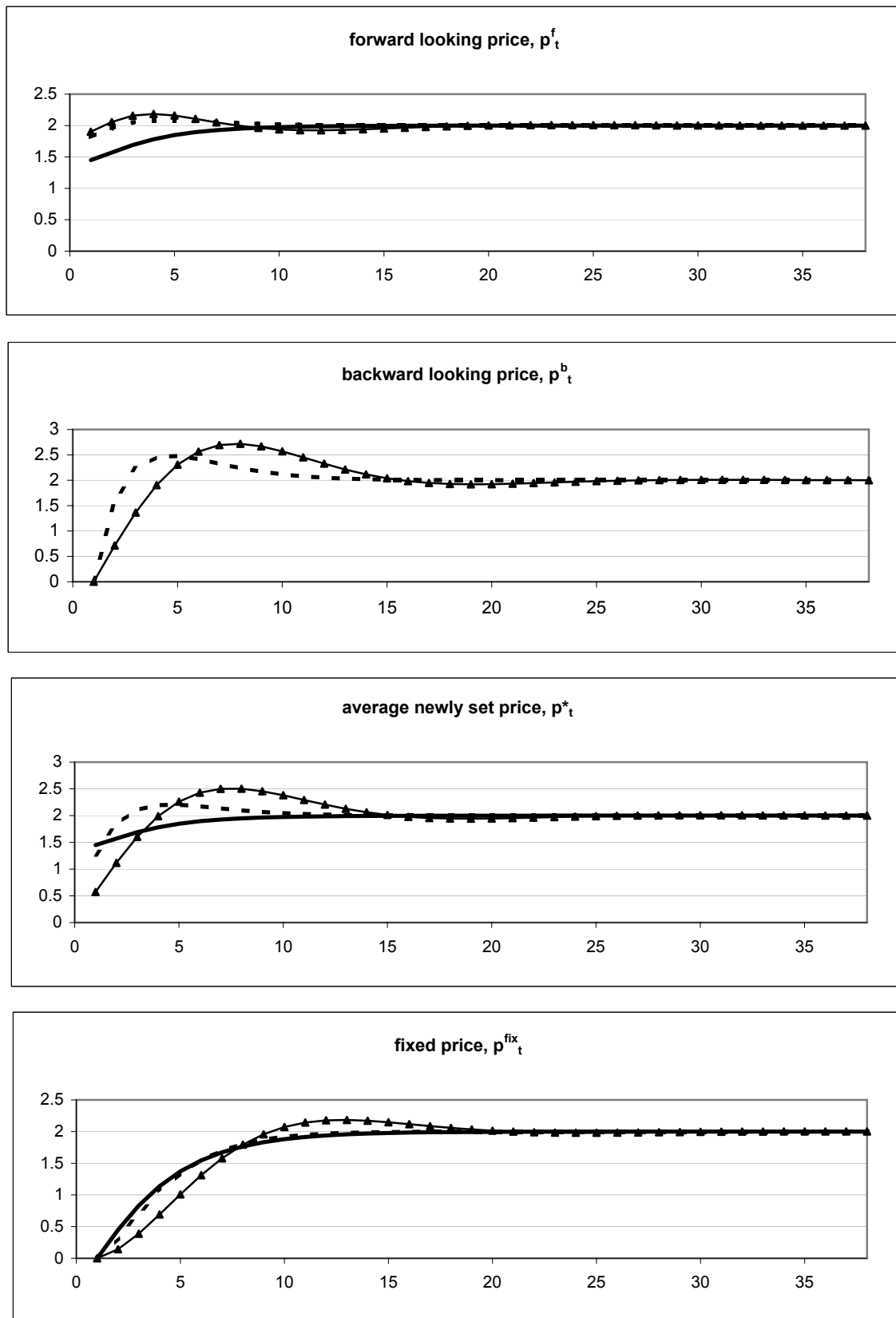
Figure 2: Impulse Response: Price Setting
