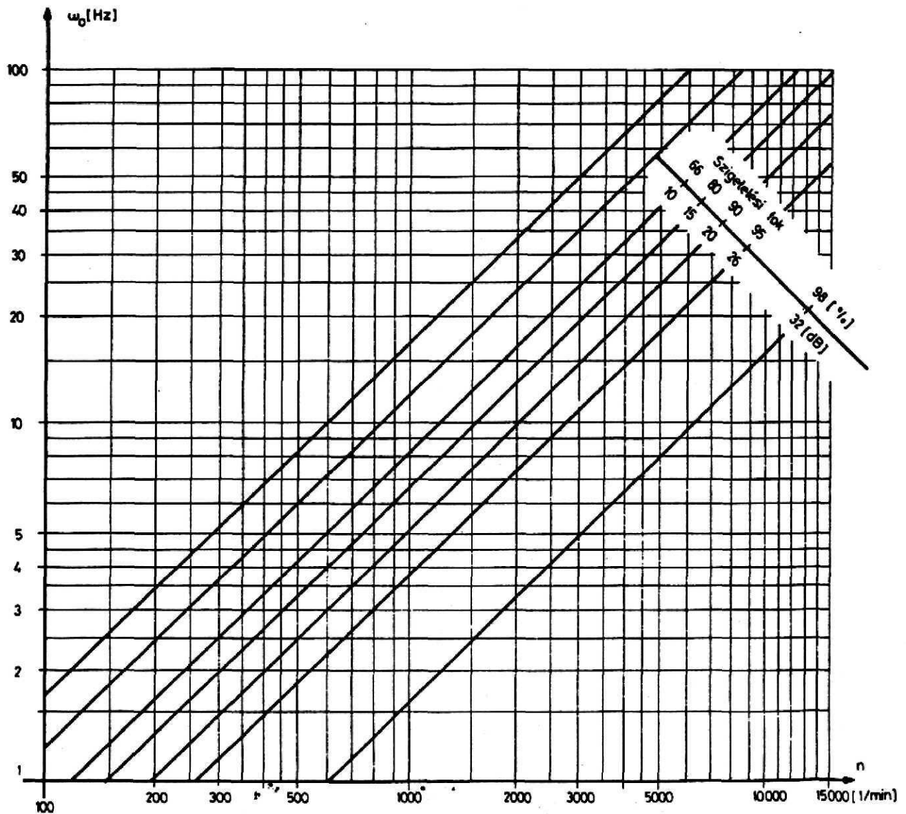
10. diagram n = \omega \cdot \frac{30}{\pi} [1/min]
