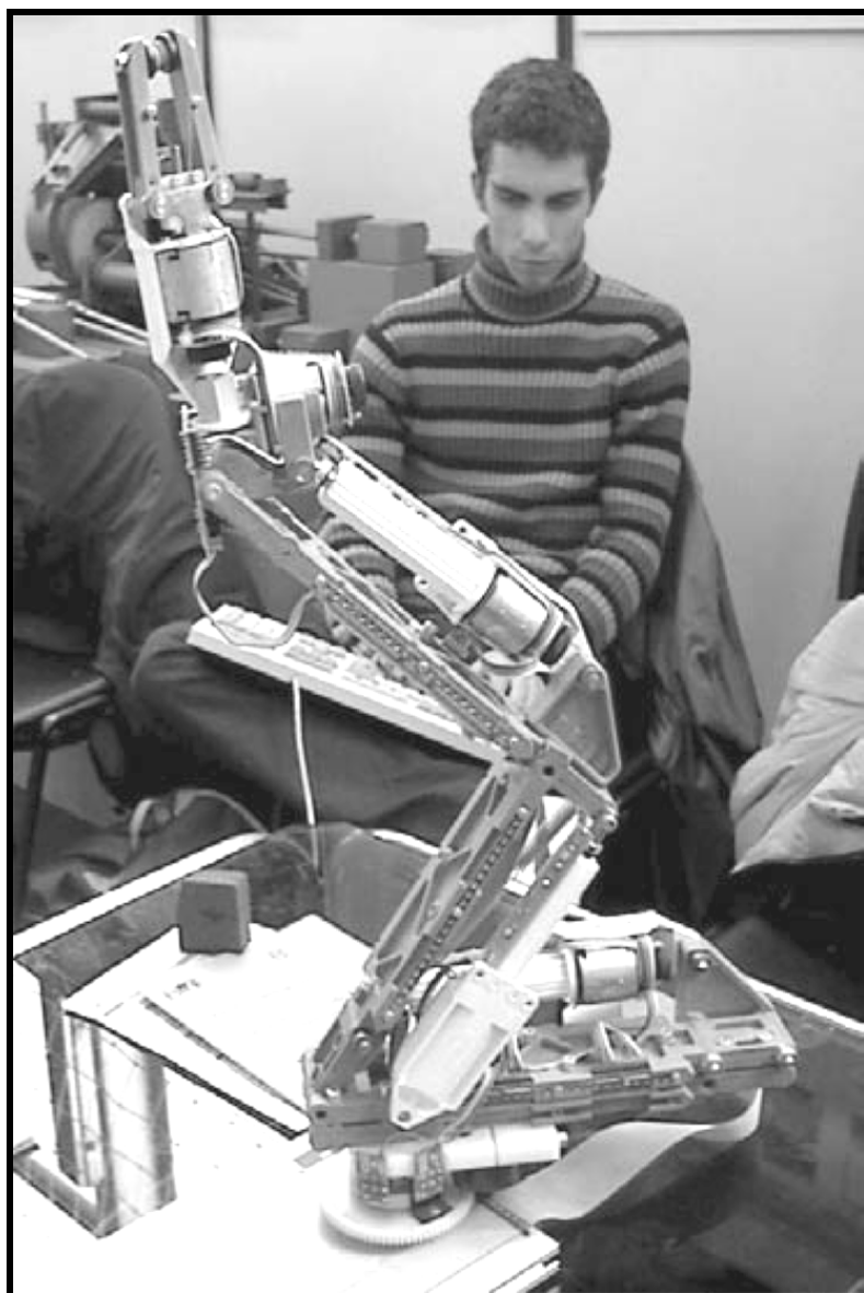
Laborgyakorlat robottal
