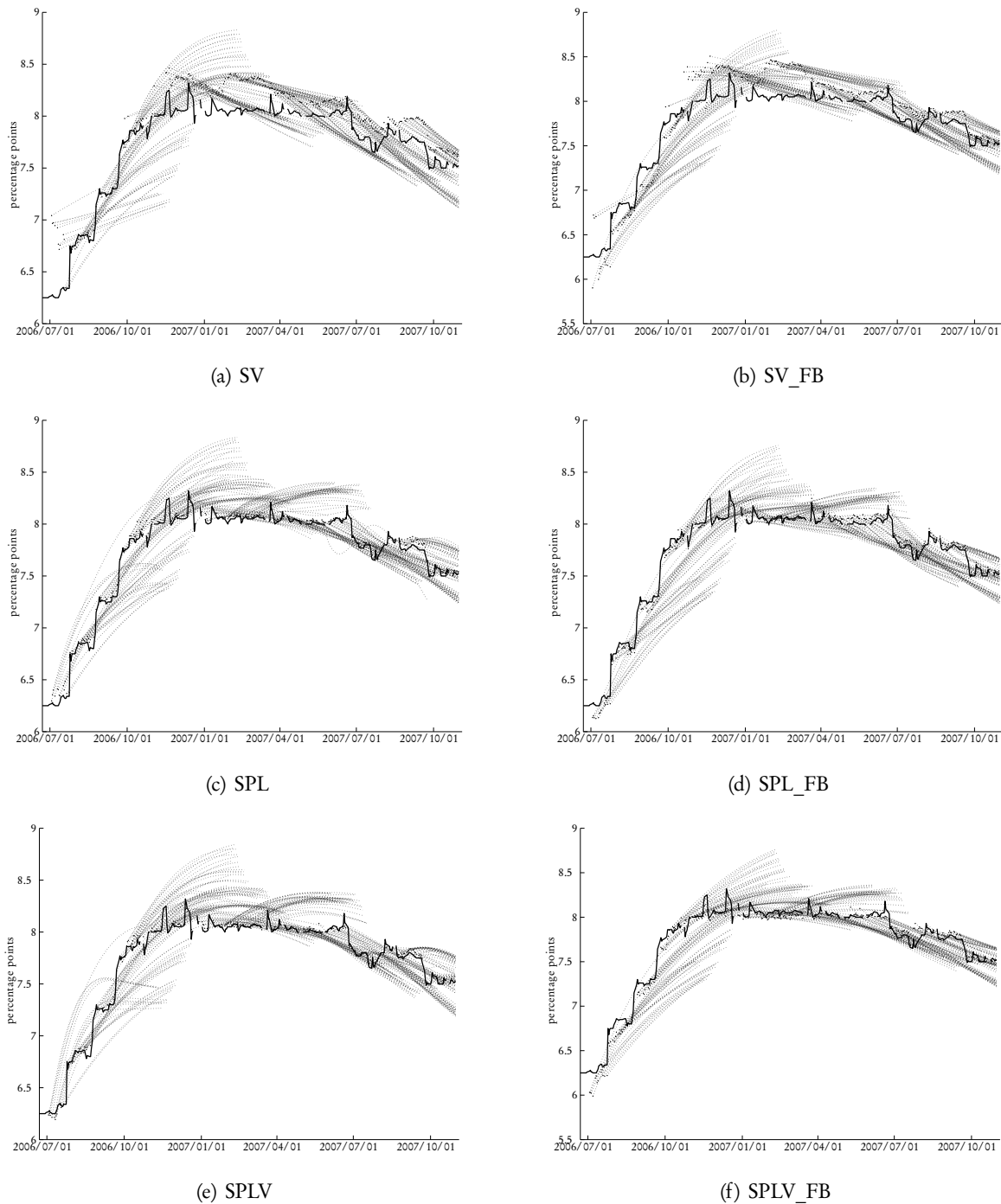
Figure 7 Short rates
