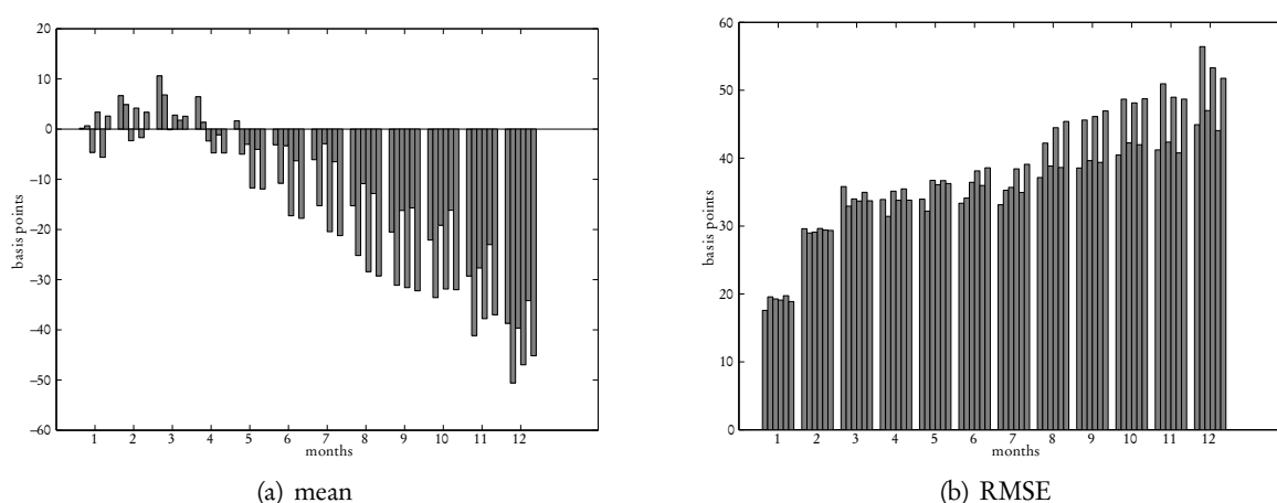
Figure 6 Forecast errors
